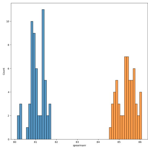
(b) all-MiniLM-l6-v2
