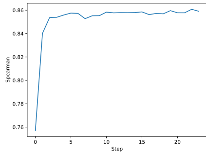
(b) all-MiniLM-l6-v2
