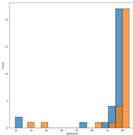
(a) bert-base-uncased
