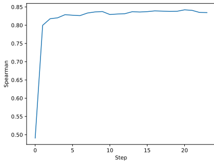
(a) bert-base-uncased
